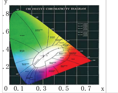
CIE1931 CHROMATICITY DIAGRAM
